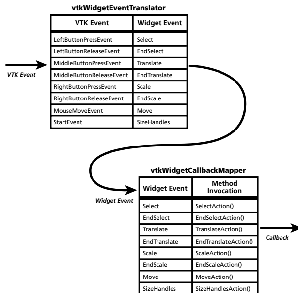
Figure 4: Widget event translation.
