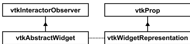
Figure 3: Overview of VTK widget design.
